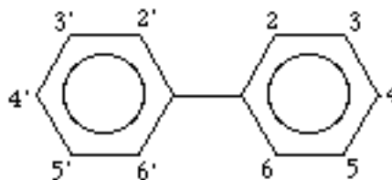
Figure 1: Basic Chemical Structure of PCBs
